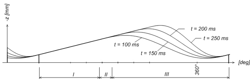
Figure 7. Family of curves defined by event-driven Flex Profile, z-axis. Sealing times of t = 100 ms, 150 ms, 200 ms and 250 ms (default) are shown.
