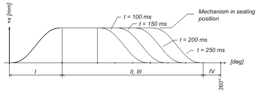
Figure 6. Family of curves defined by event-driven Flex Profile, x-axis. Sealing times of t = 100 ms, 150 ms, 200 ms and 250 ms (default) are shown.
