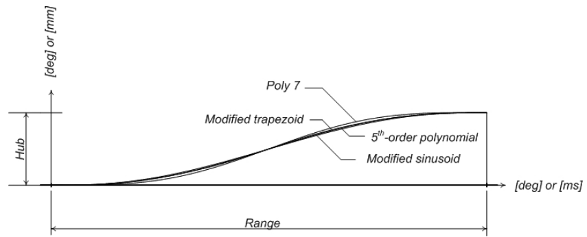
Figure 4. Standard segment, various motion laws shown. Standard segments may be synchronous or time-based. Synchronous and time-based steps, together with the Flex segments defined below, may be combined to form a final Flex Profile.
