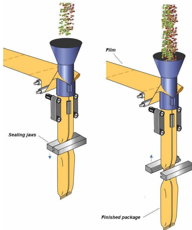
Figure 1. Steps in the production of a vertical form-fill-seal package.
