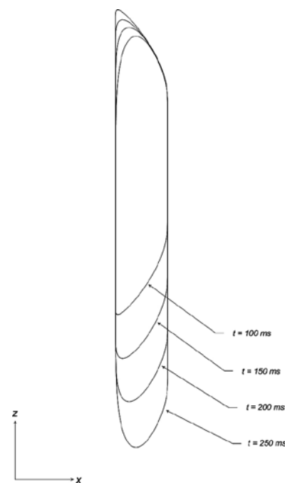
Figure 8. Sample of trajectories generated by Flex Profile as a function of the sealing time t . Note that the trajectory is calculated in-process and that the event which signals the end of sealing may occur at any time during the sealing process.
