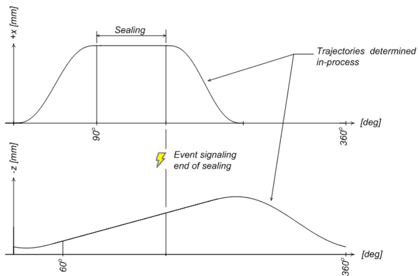
Figure 3. In the event-driven motion model, the sealing bars open as soon as the event occurs and (after some overlap) the bars return to their start position. Note that in this scheme the return trajectory is not predetermined as the event may occur at any time.
