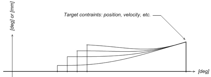
Figure 5. Flex segments are defined by the target constraints. The final trajectory is determined automatically at run-time. Trajectories for various initial conditions are shown.
