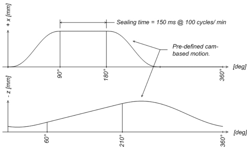
Figure 2. Cam profiles based on an assumed master speed of 100 cycles/minute. In this case, to achieve a sealing time of t = 150 ms, sealing is defined to occur between 90 degrees and 180 degrees of the master cycle.
